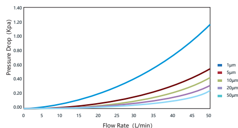
BDLB Filter Pressure Drop vs Flow Rate @20C
