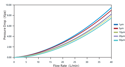
BDLS Filter Pressure Drop vs Flow Rate @20°C
